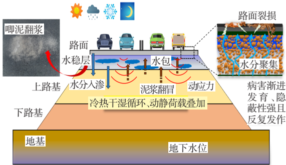
图9 复杂运营环境增大道路翻浆病害发生风险示意图 Figure 9 Mud pumping risk increased by complex operating environment
