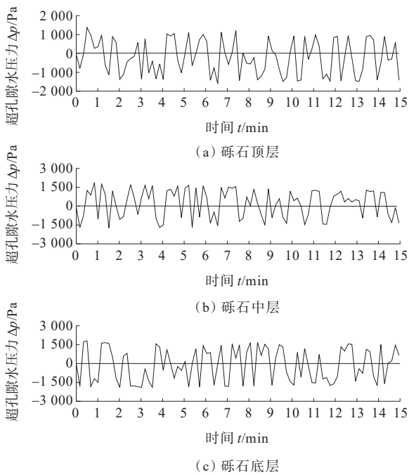
图3 砾石层不同深度处超孔隙水压力随时间的变化 Figure 3 Variation of excess pore pressure with time at different gravel layer depths
