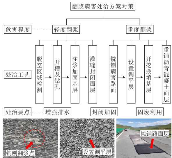
图10 高原公路翻浆病害处治思路与方案 Figure 10 Approach and solution for treating mud pumping on plateau highway
