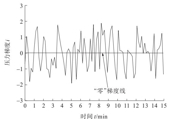
图4 砾石层内压力梯度随时间变化 Figure 4 Variation of pressure gradient in gravel layer with time
