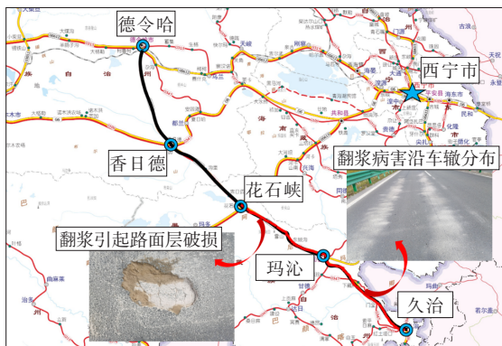
图7 G0615德马高速(花石峡至久治段)翻浆实地调研 Figure 7 Field investigation on mud pumping on G0615 Dema Expressway (Huashixia to Jiuzhi Section)
